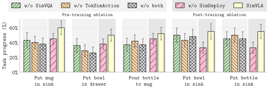
Figure 6. Averaged task progress across tasks in mock kitchen-ID. Removing either SimVQA or Tokenized SimAction degrades performance across all tasks. SimDeploy yields task-dependent gains in zero-shot deployment performance.
