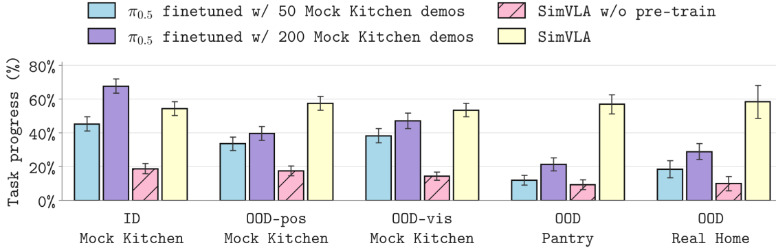
Figure 5. Averaged task progress in real-world environments. Mock kitchen includes all five tasks; pantry includes put mug / bowl / bottle in sink ; real home includes put mug in sink / pour bottle to mug . SimVLA maintains robust performance in OOD environments, while the fine-tuned policy degrades substantially. Removing pre-training leads to poor performance, demonstrating its importance for robust generalization.
