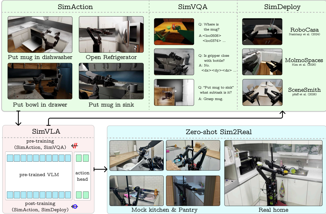
Figure 1. SimVLA: Zero-shot sim-to-real framework for mobile manipulation.
