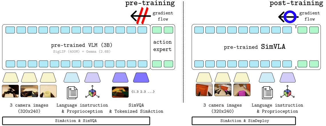
Figure 2. Overview of SimVLA Training. During pre-training, SimVLA jointly optimizes continuous action prediction, tokenized action prediction, and SimVQA supervision. During post-training, SimVLA is trained on a mixture of SimAction actions and deployment trajectories from SimDeploy.
