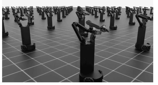
Figure 13. Massive parallel environments (4096 instances) running simultaneously in Isaac Lab for hybrid system identification.
